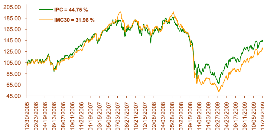
IPC and IMC30 Behavior in Dollars in Base 100 Dec 30th, 2005 - Nov 30th, 2009
